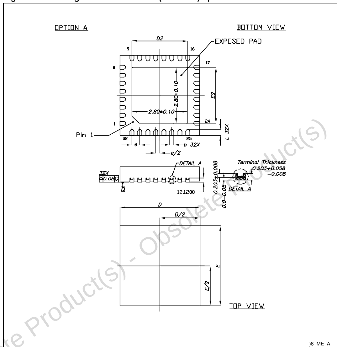
Figure 26. Package outline for QFN32 (4 x 4 mm) - pitch 0.4 mm
