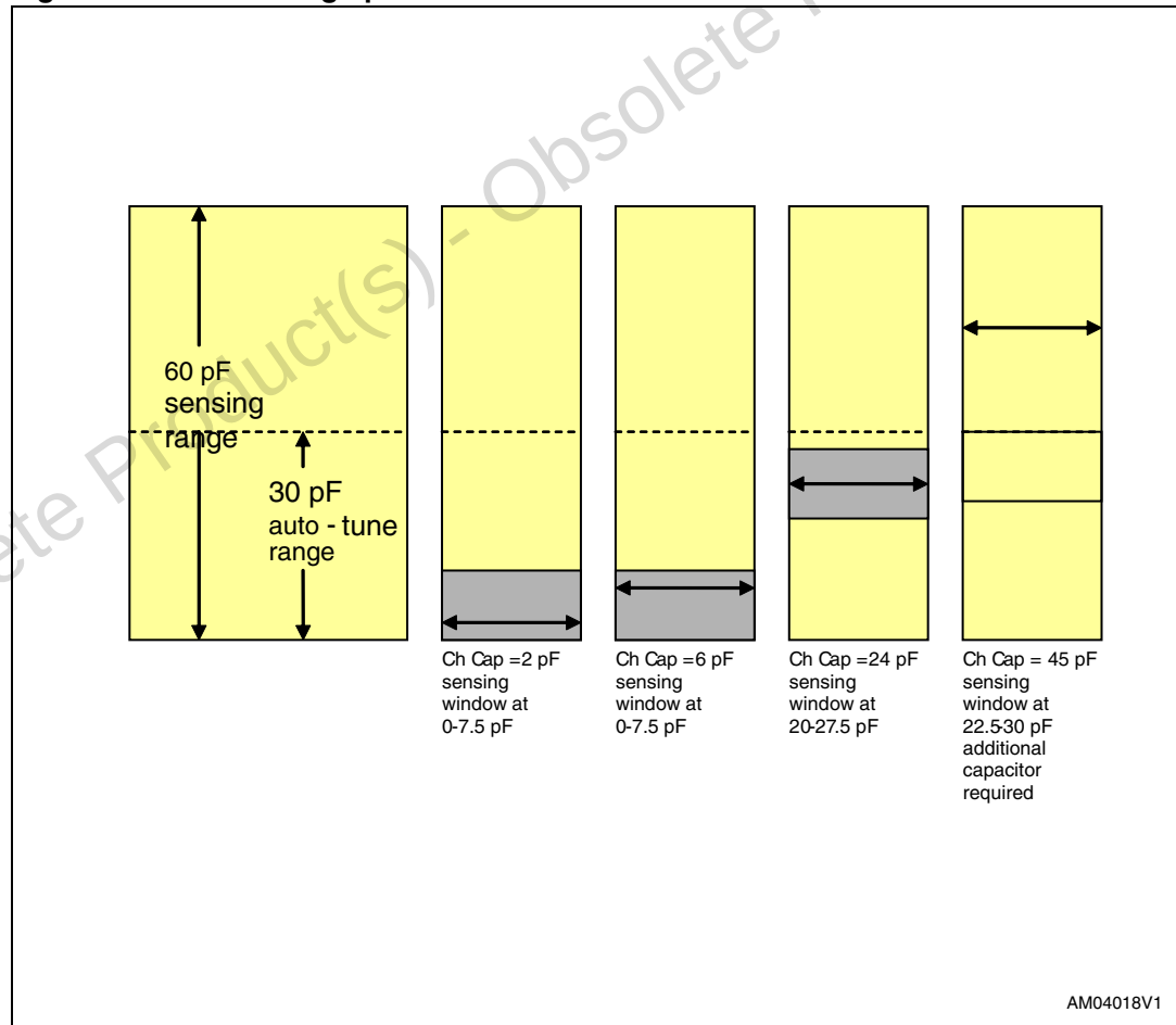
Figure 15. Auto-tuning operation
